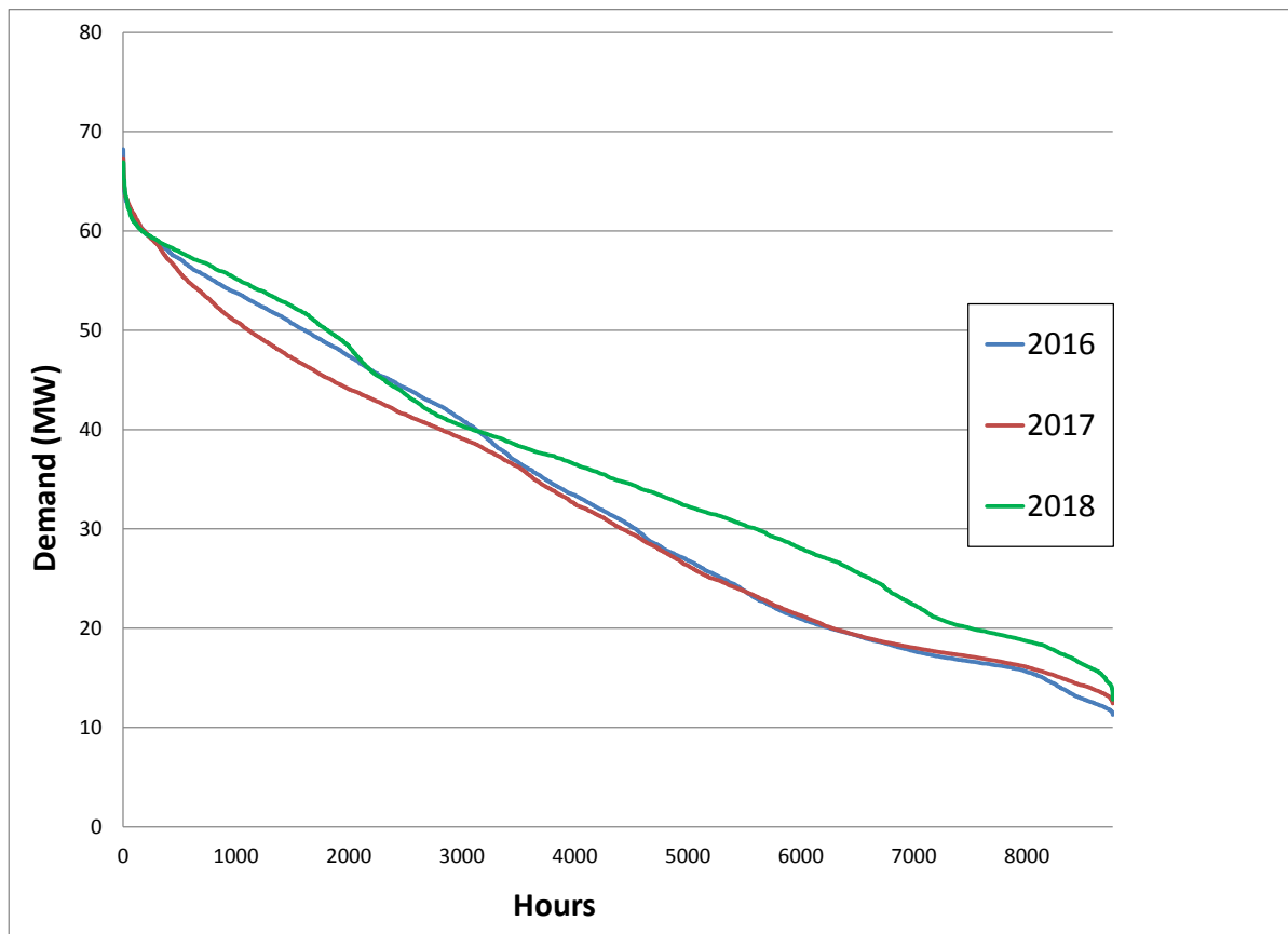
Figure 1: Labrador East Transmission System Load Duration Curves (2016, 2017, and 2018)
