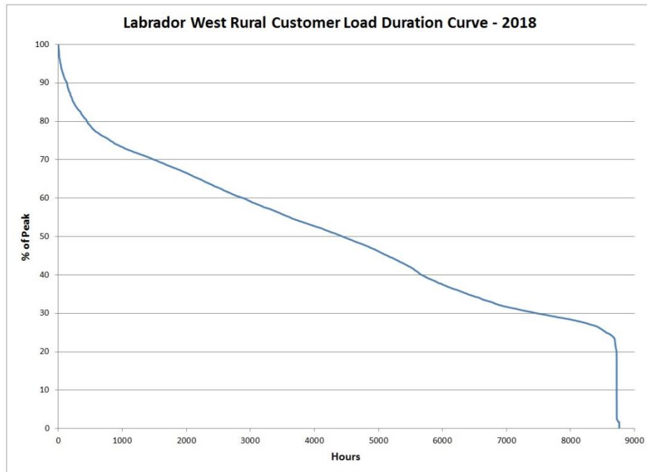
Figure 9: Labrador West Rural Customer Load Duration Curve for 2018
