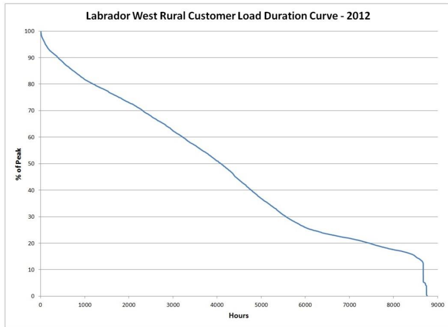
Figure 3: Labrador West Rural Customer Load Duration Curve for 2012
