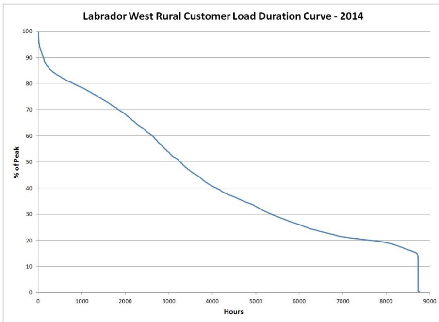
Figure 5: Labrador West Rural Customer Load Duration Curve for 2014
