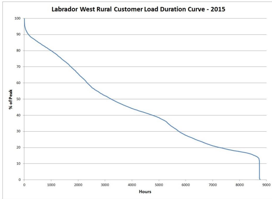
Figure 6: Labrador West Rural Customer Load Duration Curve for 2015
