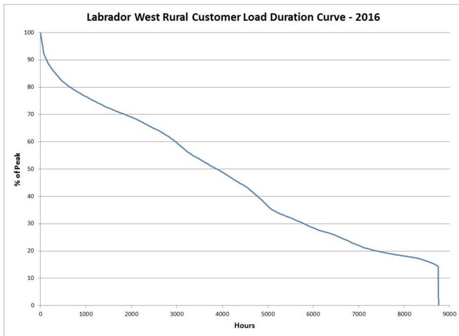
Figure 7: Labrador West Rural Customer Load Duration Curve for 2016
