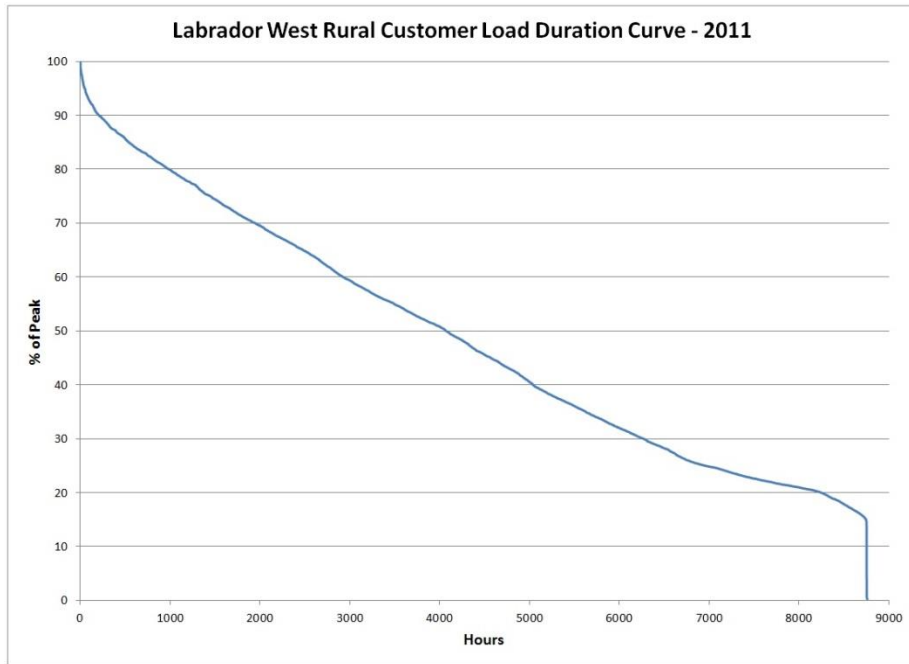
Figure 2: Labrador West Rural Customer Load Duration Curve for 2011
