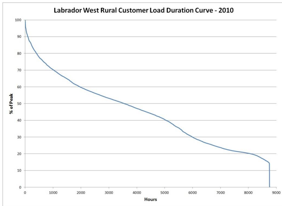
Figure 1: Labrador West Rural Customer Load Duration Curve for 2010
