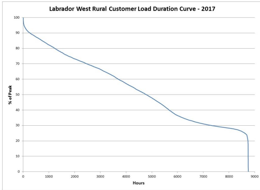
Figure 8: Labrador West Rural Customer Load Duration Curve for 2017
