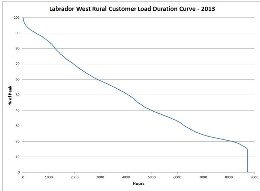
Figure 4: Labrador West Rural Customer Load Duration Curve for 2013
