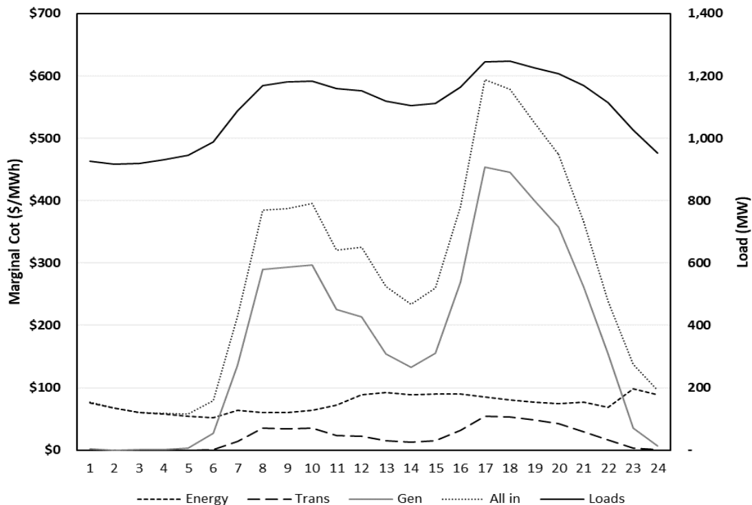
Figure 12: JANUARY 2021 AVERAGE HOURLY MARGINAL COSTS AND LOADS
