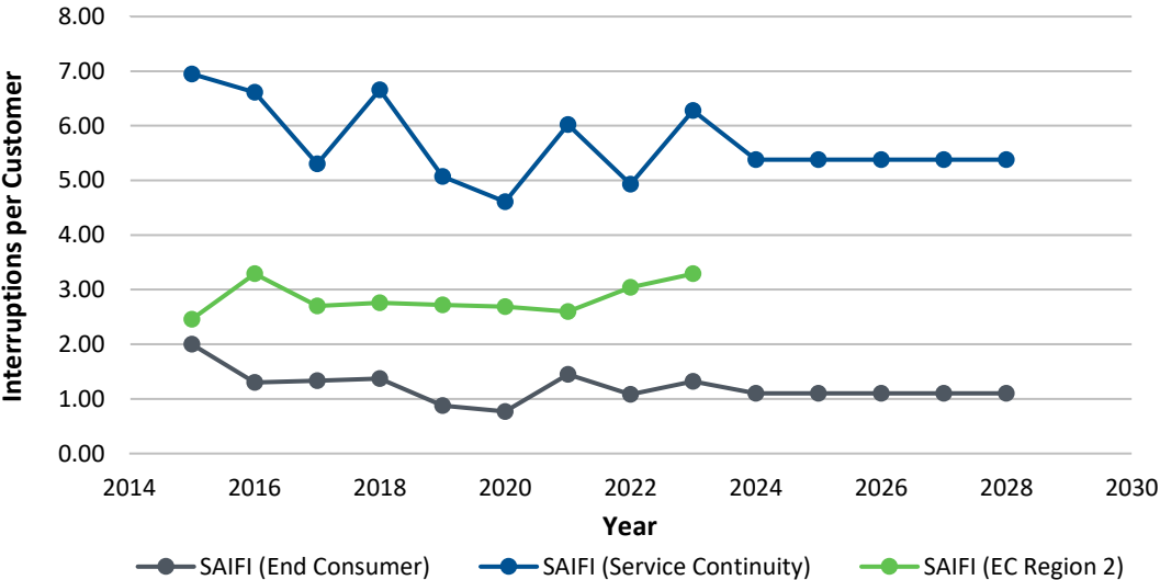
Chart 2: SAIFI Excluding Major Events
