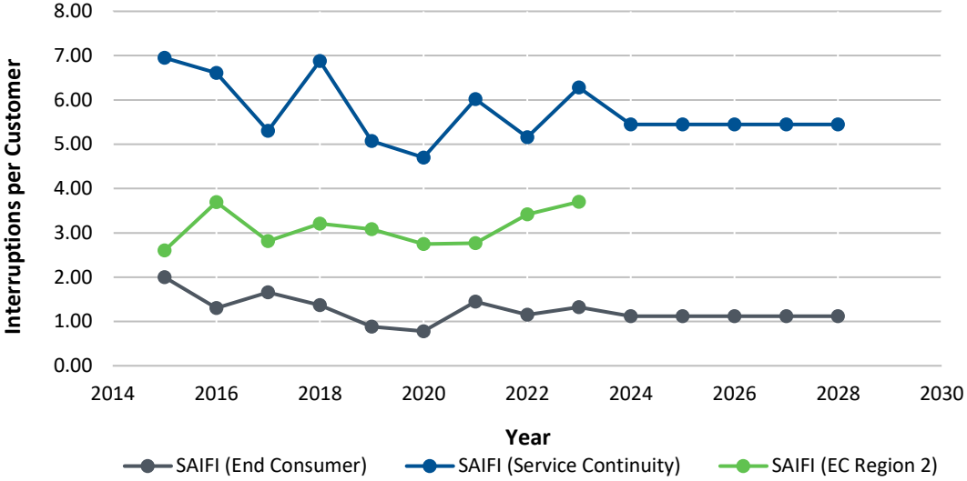
Chart 3: SAIFI Including Major Events
