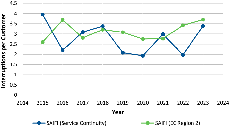
Chart 11: SAIFI Including Major Events – Labrador
