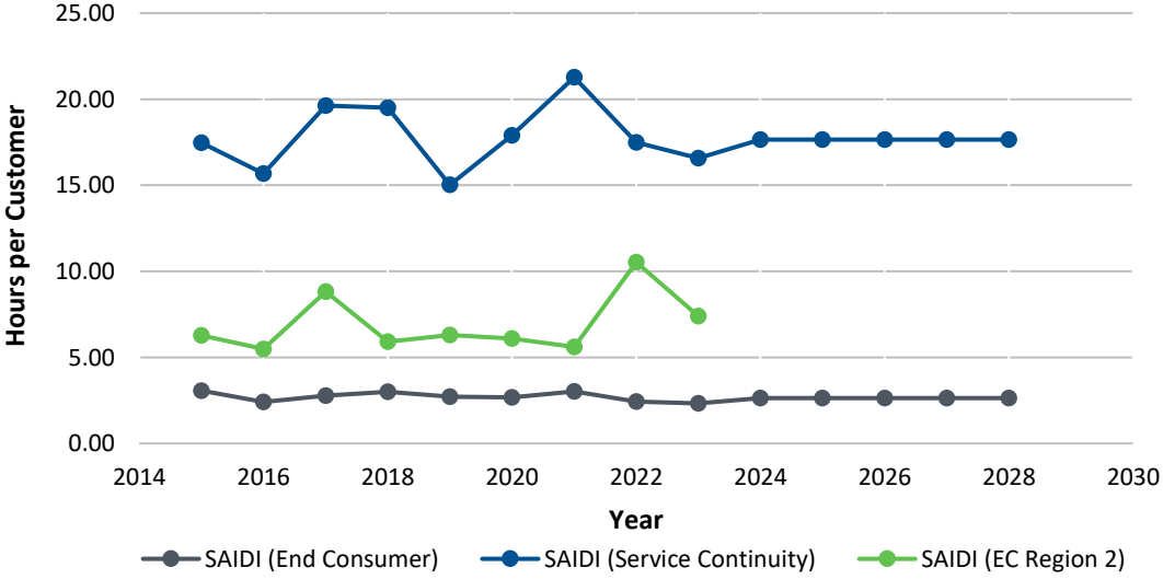
Chart 4: SAIDI Excluding Major Events
