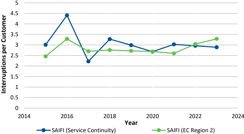
Chart 6: SAIFI Excluding Major Events – Island
