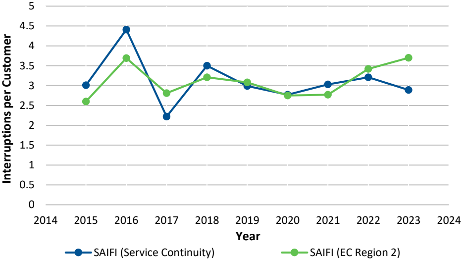
Chart 7: SAIFI Including Major Events – Island
