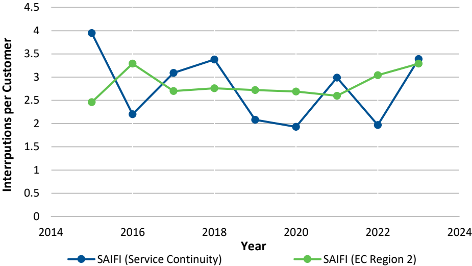
Chart 10: SAIFI Excluding Major Events – Labrador
